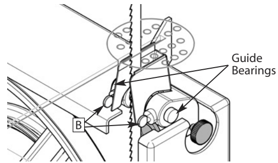
Figure 18 - Basic alignment.
