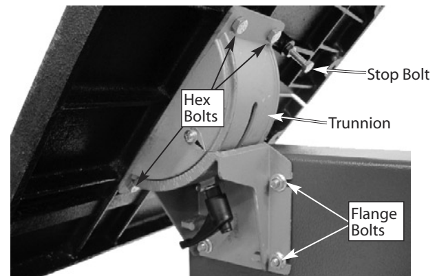
Figure 1 - Assemble table to trunnion.
