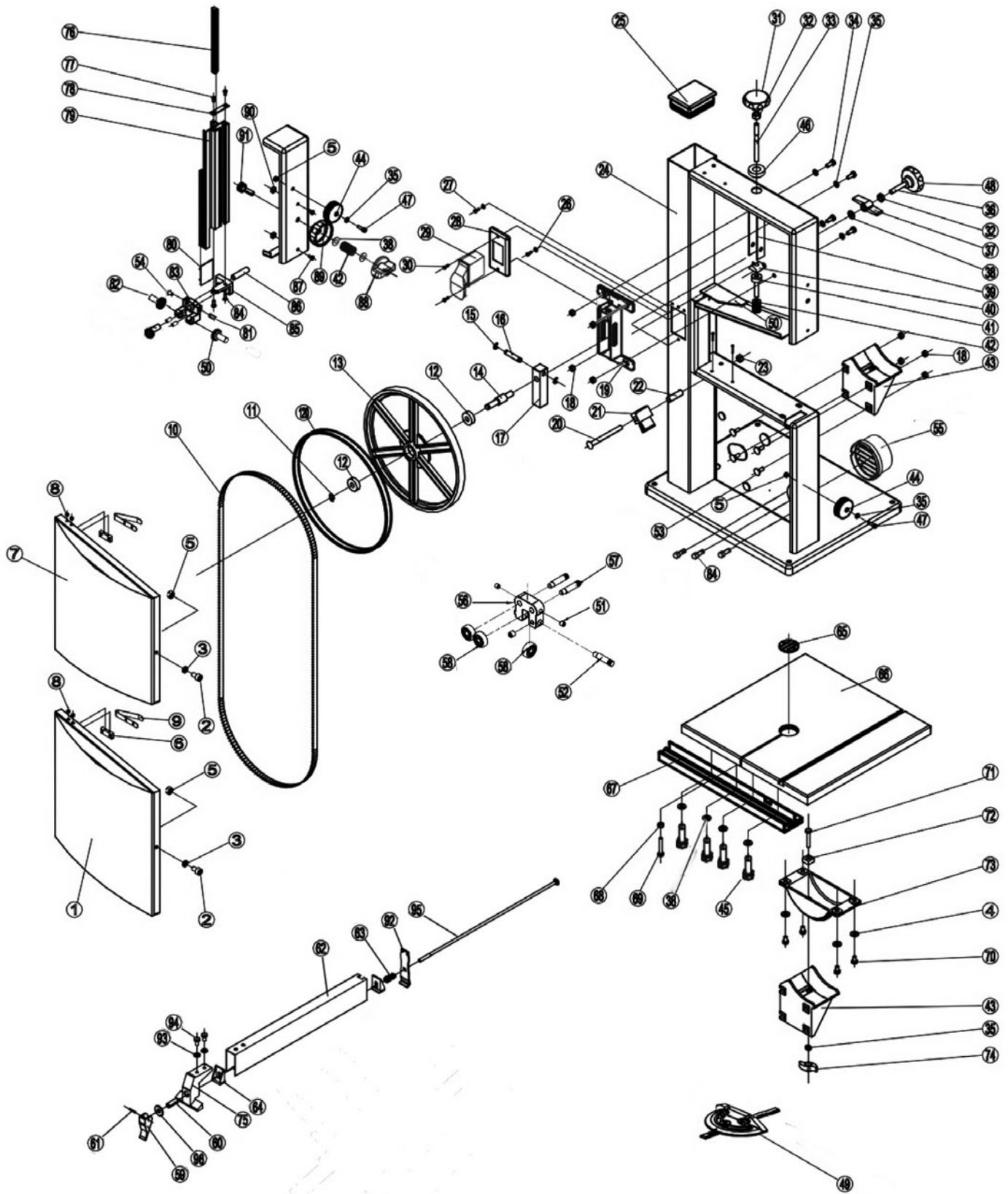
Figure 21 - Replacement parts illustration for 10" Bench Top Band Saw.
