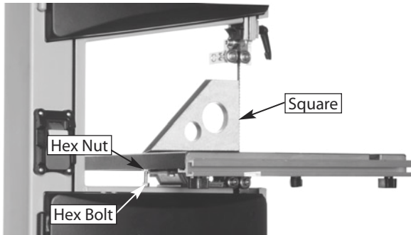
Figure 2 - Square table to saw blade.
