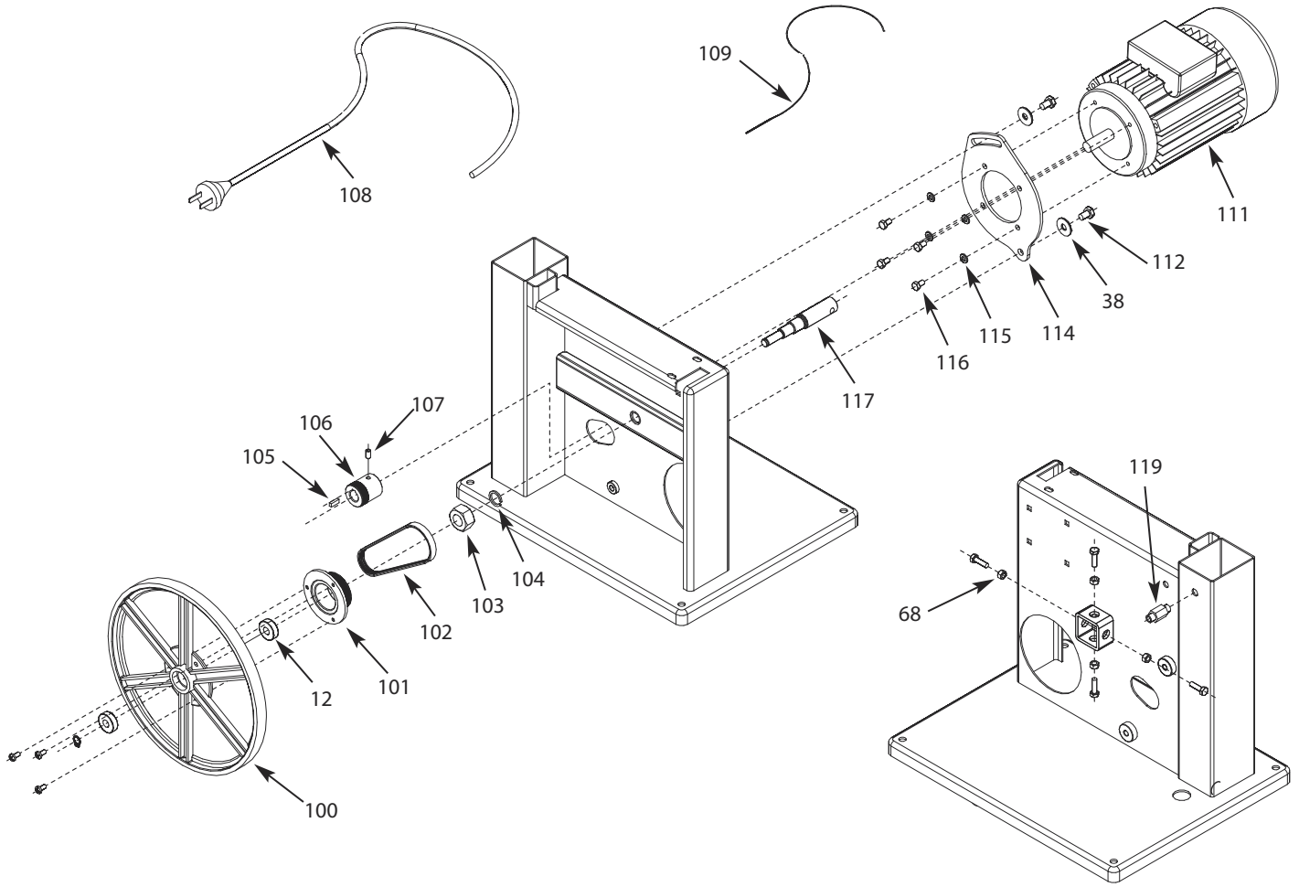
Figure 23 - Replacement parts illustration for 10" Bench Top Band Saw (continued).
