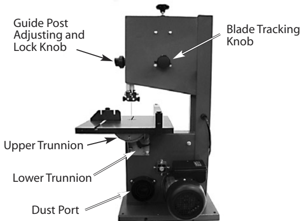
Figure 8 - Know your band saw.
