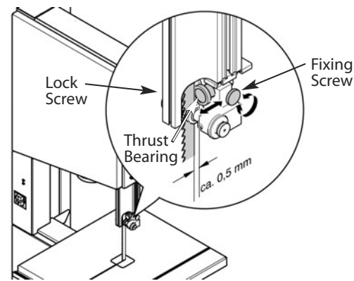
Figure 14 - Adjusting the thrust bearings.
