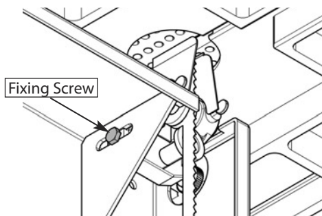
Figure 16 - Basic alignment.
