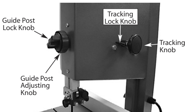
Figure 13 - Set tracking of saw blade.
