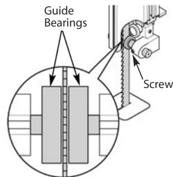
Figure 15 - Adjusting the guide bearings.
