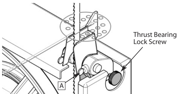
Figure 17 - Basic alignment.
