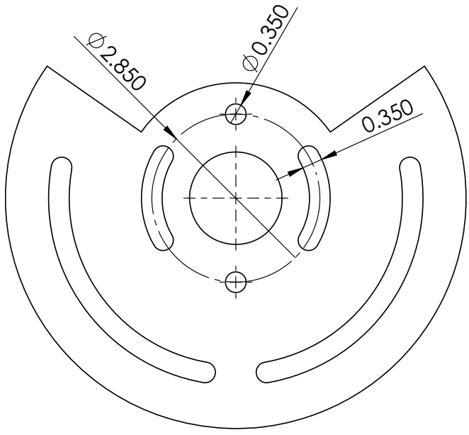
Figure 1 – Mounting bracket.
