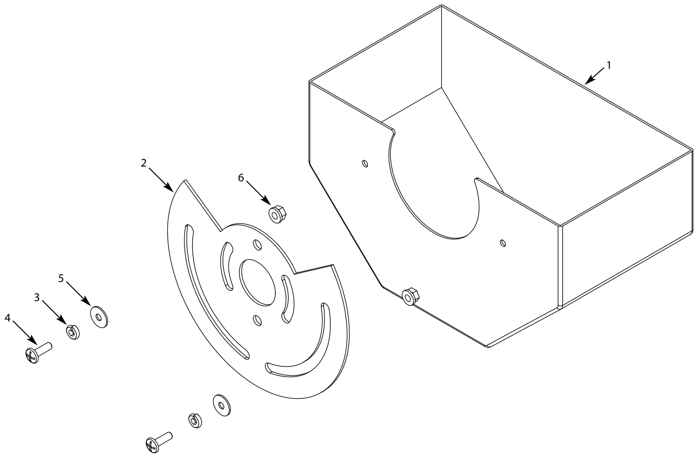
Figure 2 – Repair parts illustration for 9682099 buffer guard.
